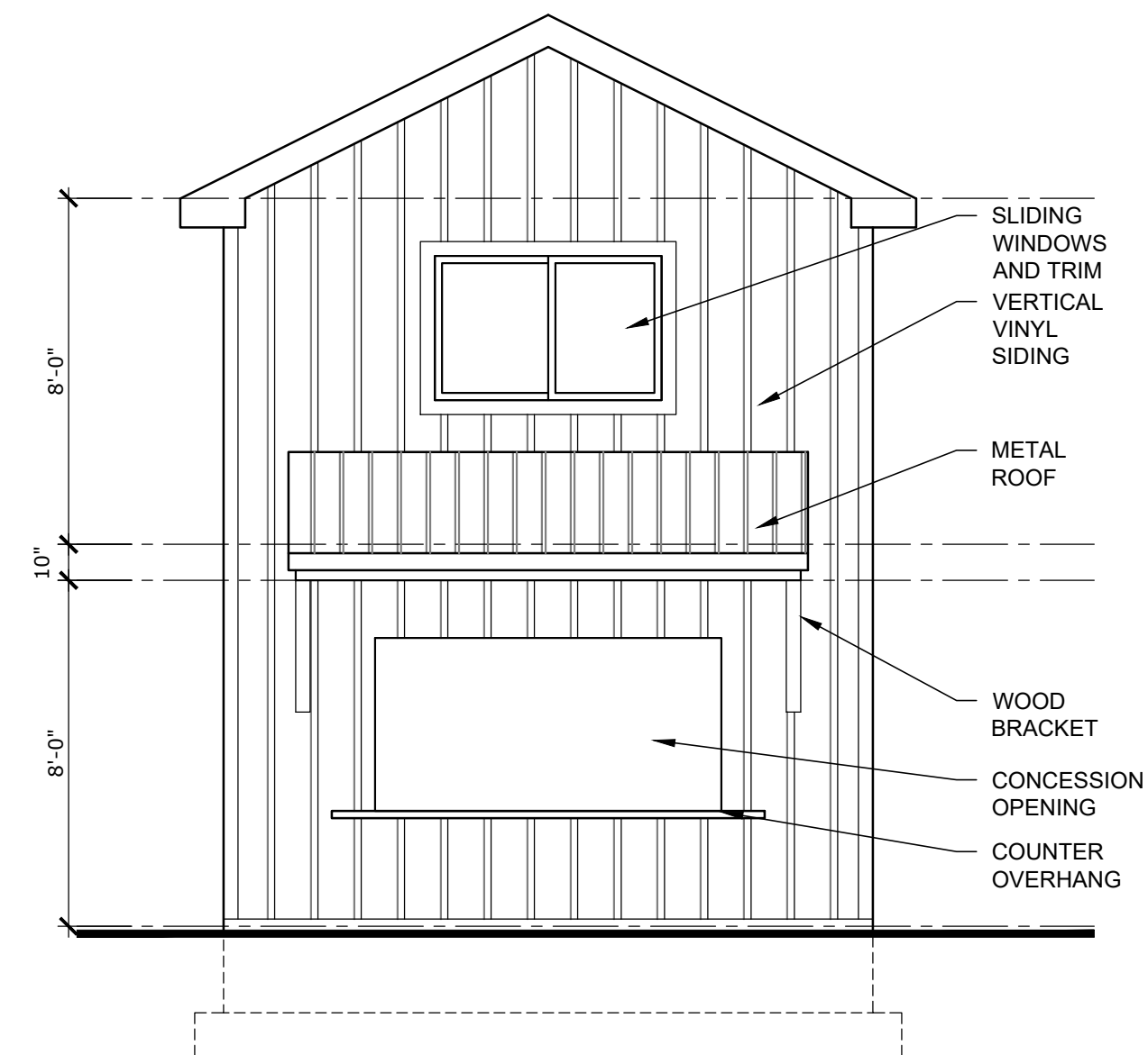
4 SIDE ELEVATION 1/4" = 1'-0"
