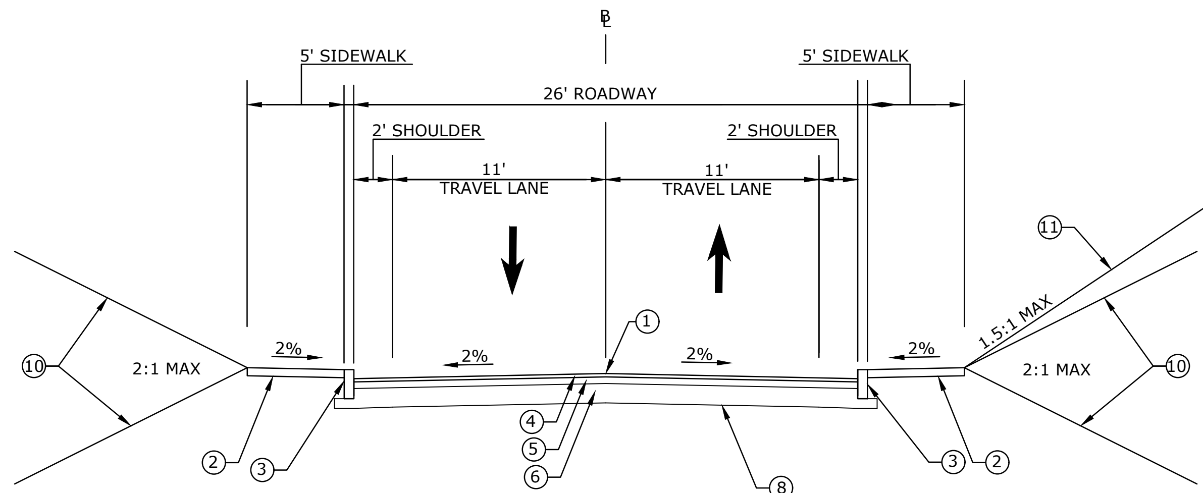
DIVISION STREET NORMAL ROADWAY SECTION (NOT TO SCALE)
