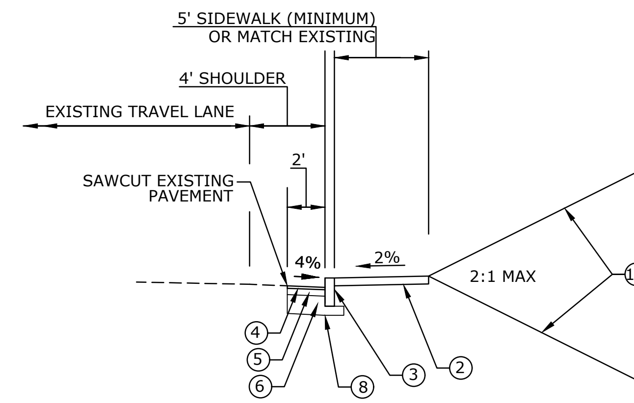
DIVISION ST, SEYMOUR AVE, MAPLE AVE PARTIAL SECTION CONCRETE CURBING AND SIDEWALK (NOT TO SCALE)
