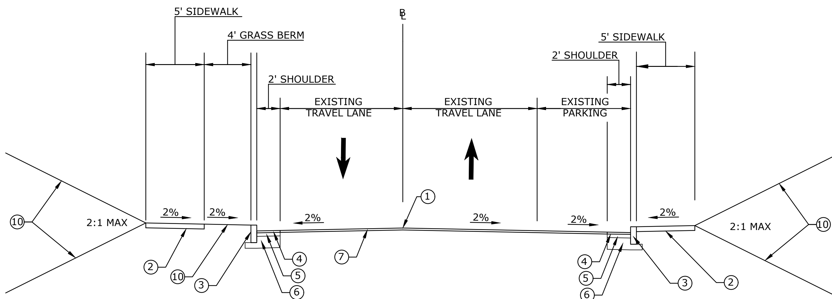
SEYMOUR AVENUE NORMAL ROADWAY SECTION (NOT TO SCALE)
