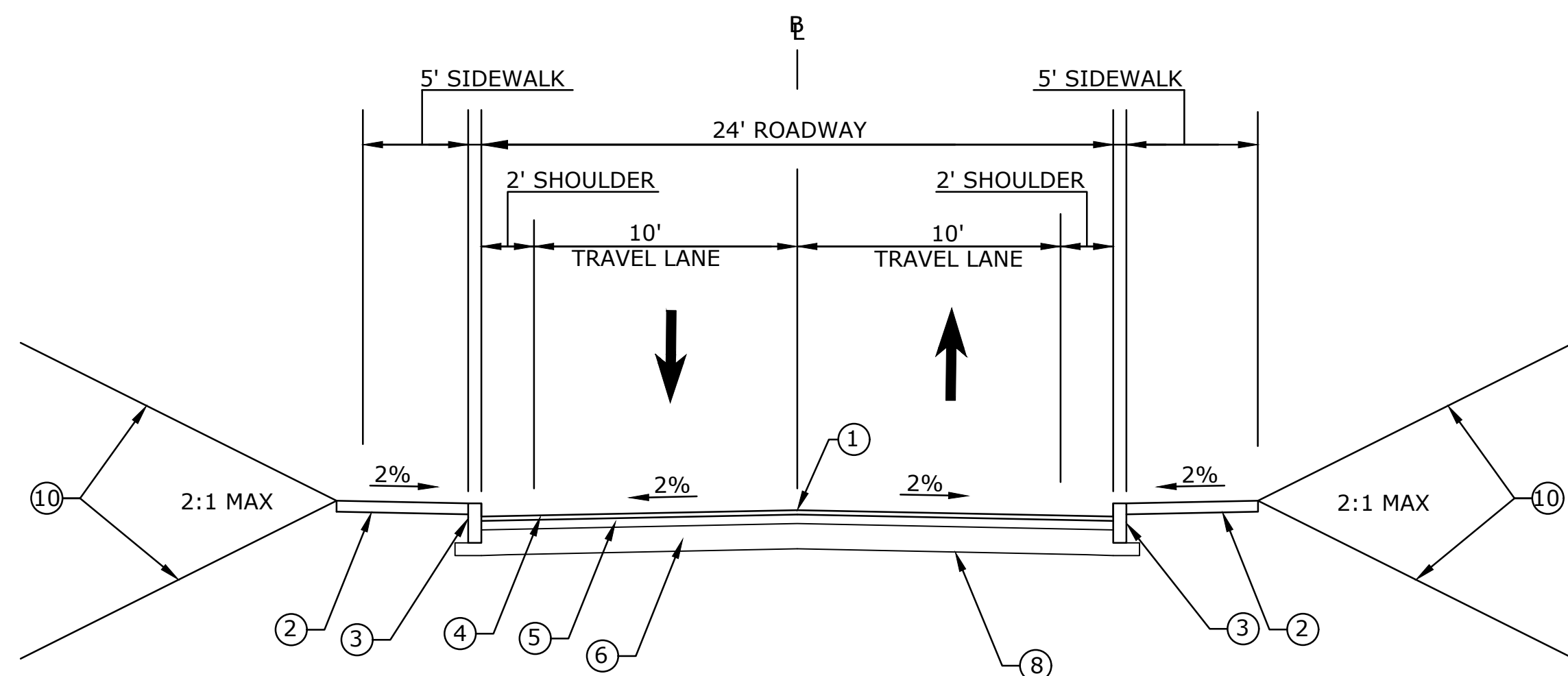
SILVER HILL ROAD NORMAL ROADWAY SECTION (NOT TO SCALE)
